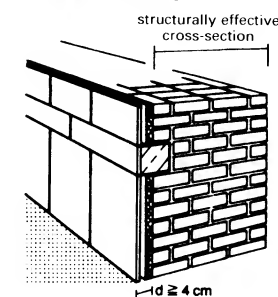
⑩ Stone cladding: structurally ineffective
